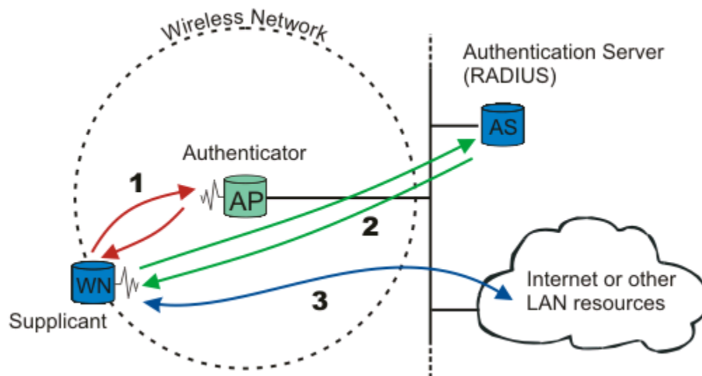
Figure 802.1X: A wireless node must be authenticated before it can gain access to other LAN resources.
